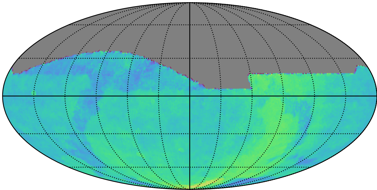
too_elab_r32_d2_gz_v3.4_10yrs All sky: Parallax Coverage @ 22.4
