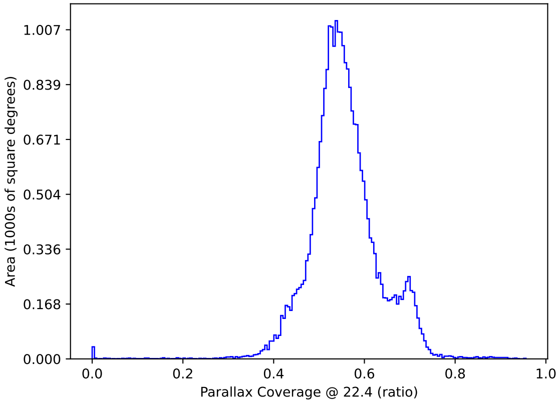
too_elab_r32_d2_gz_v3.4_10yrs All sky: Parallax Coverage @ 22.4
