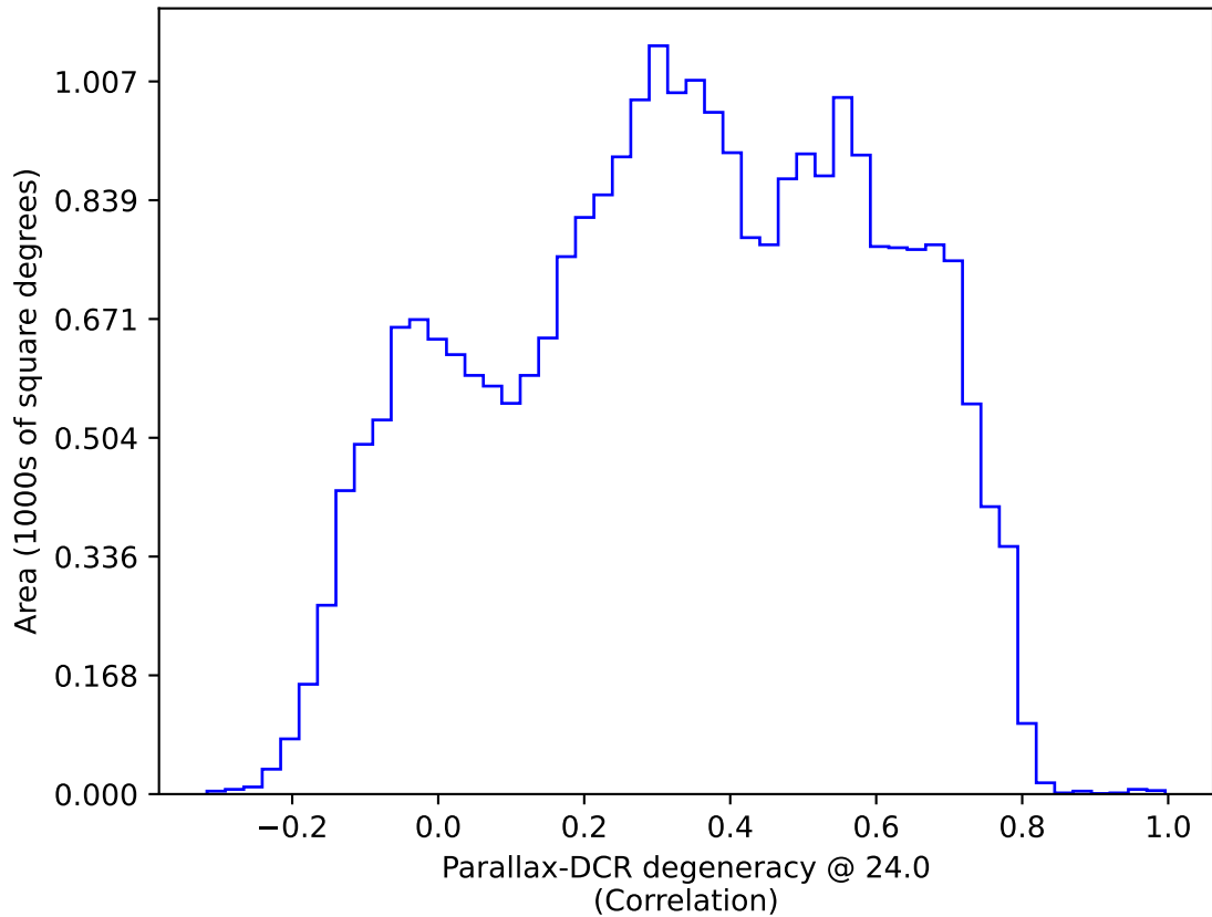
too_elab_r32_d2_gz_v3.4_10yrs All sky: Parallax-DCR degeneracy @ 24.0
