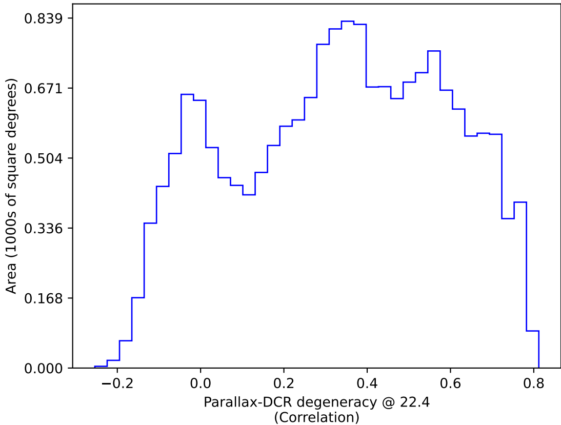
too_elab_r32_d2_gz_v3.4_10yrs WFD: Parallax-DCR degeneracy @ 22.4
