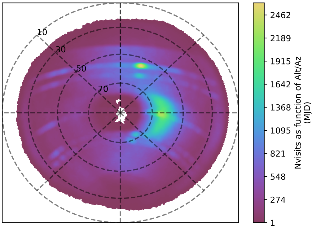
too_elab_r32_d2_gz_v3.4_10yrs z band: Nvisits as function of Alt/Az
