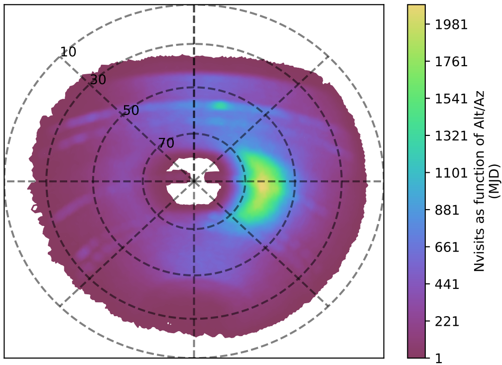
too_elab_r32_d2_gz_v3.4_10yrs y band: Nvisits as function of Alt/Az
