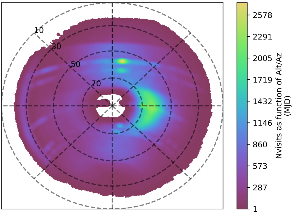
too_elab_r32_d2_gz_v3.4_10yrs r band: Nvisits as function of Alt/Az
