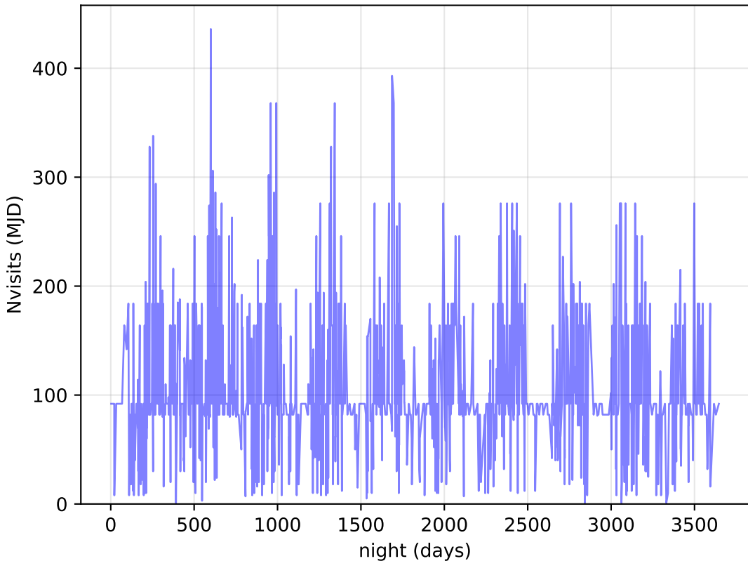
too_elab_r32_d2_gz_v3.4_10yrs DDF: Nvisits
