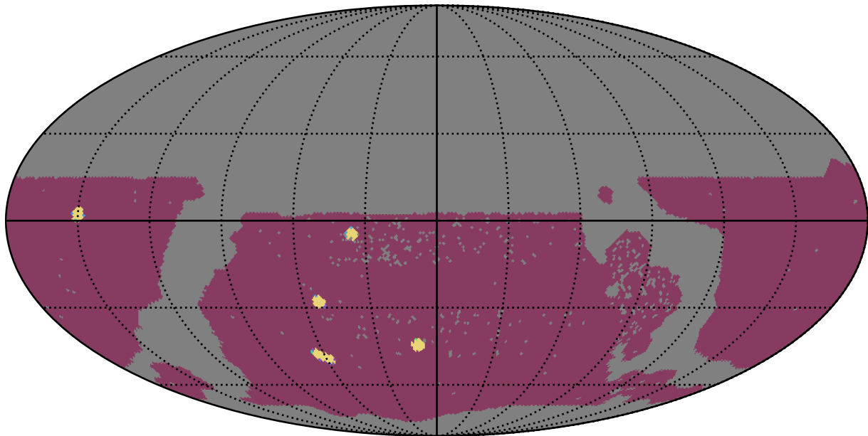
too_elab_r32_d2_gz_v3.4_10yrs WFD: NumberOfQuickRevisits
