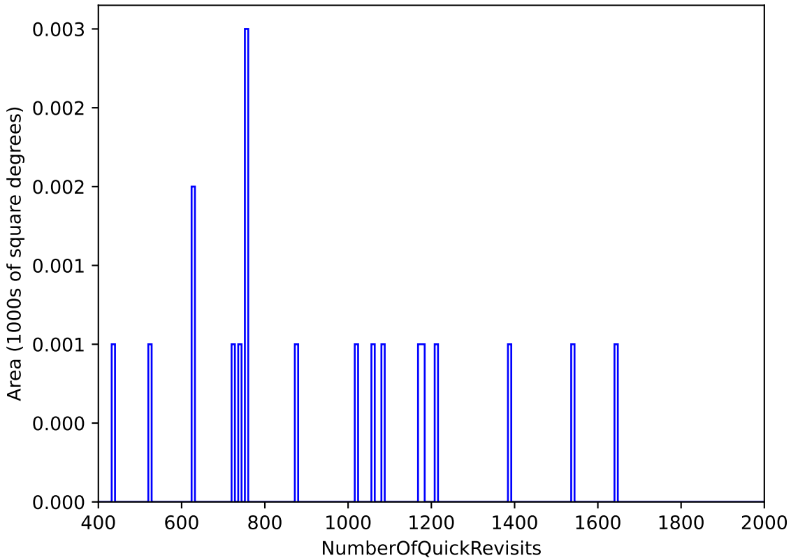
too_elab_r32_d2_gz_v3.4_10yrs WFD: NumberOfQuickRevisits
