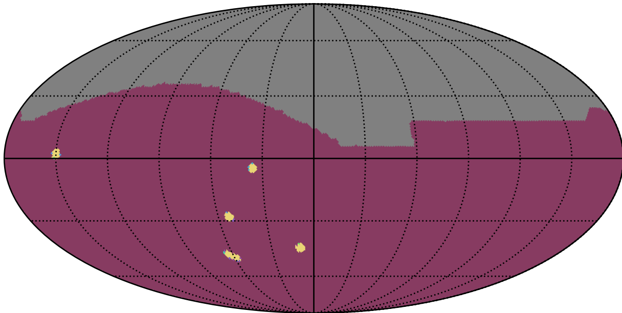
too_elab_r32_d2_gz_v3.4_10yrs All sky: NumberOfQuickRevisits
