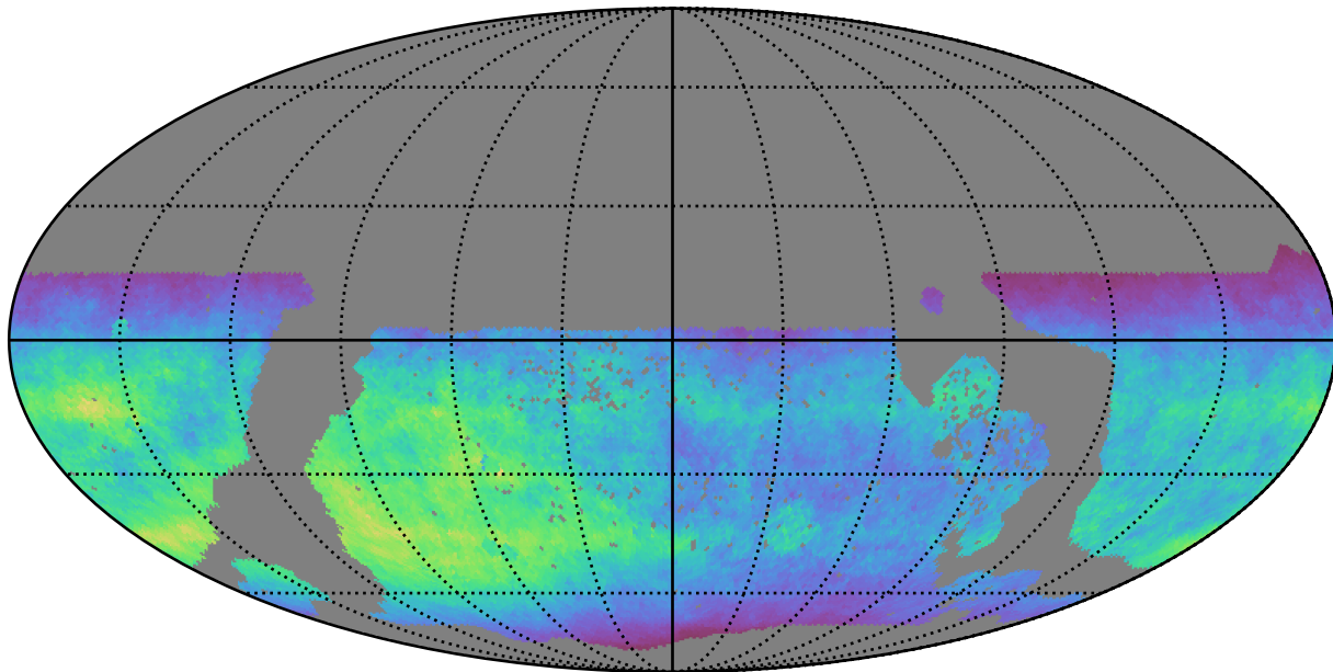
too_elab_r32_d2_gz_v3.4_10yrs WFD z band: Normalized Teff
