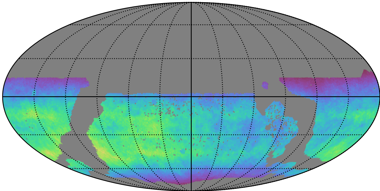
too_elab_r32_d2_gz_v3.4_10yrs WFD y band: Normalized Teff
