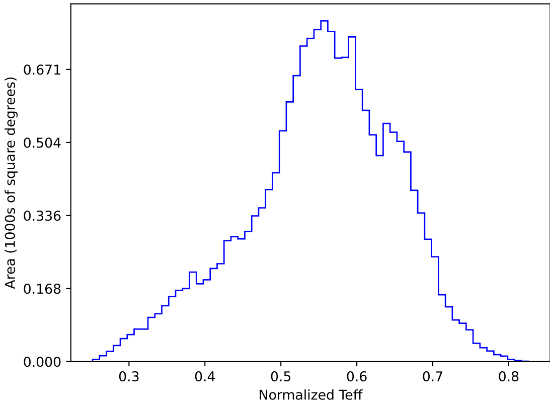
too_elab_r32_d2_gz_v3.4_10yrs WFD y band: Normalized Teff
