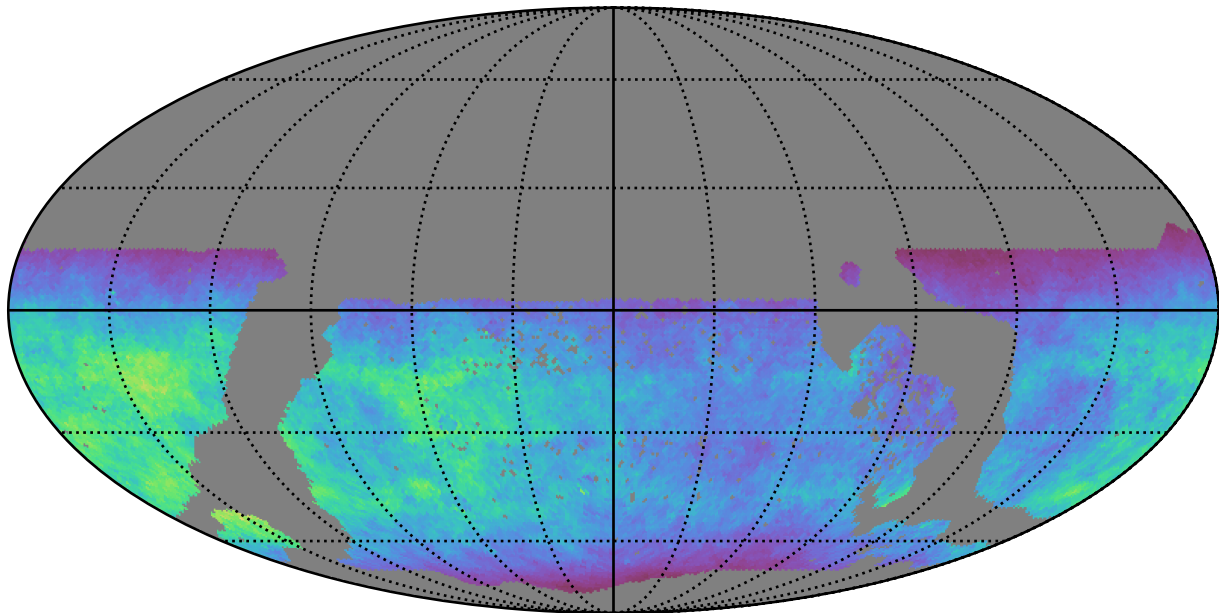
too_elab_r32_d2_gz_v3.4_10yrs WFD u band: Normalized Teff
