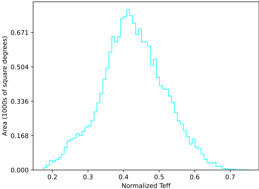
too_elab_r32_d2_gz_v3.4_10yrs WFD u band: Normalized Teff
