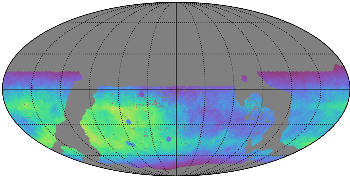
too_elab_r32_d2_gz_v3.4_10yrs WFD r band: Normalized Teff
