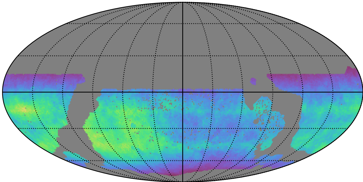
too_elab_r32_d2_gz_v3.4_10yrs WFD i band: Normalized Teff
