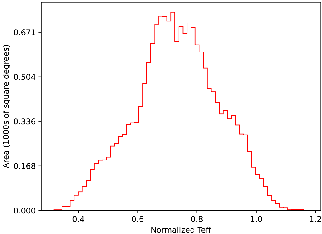
too_elab_r32_d2_gz_v3.4_10yrs WFD i band: Normalized Teff
