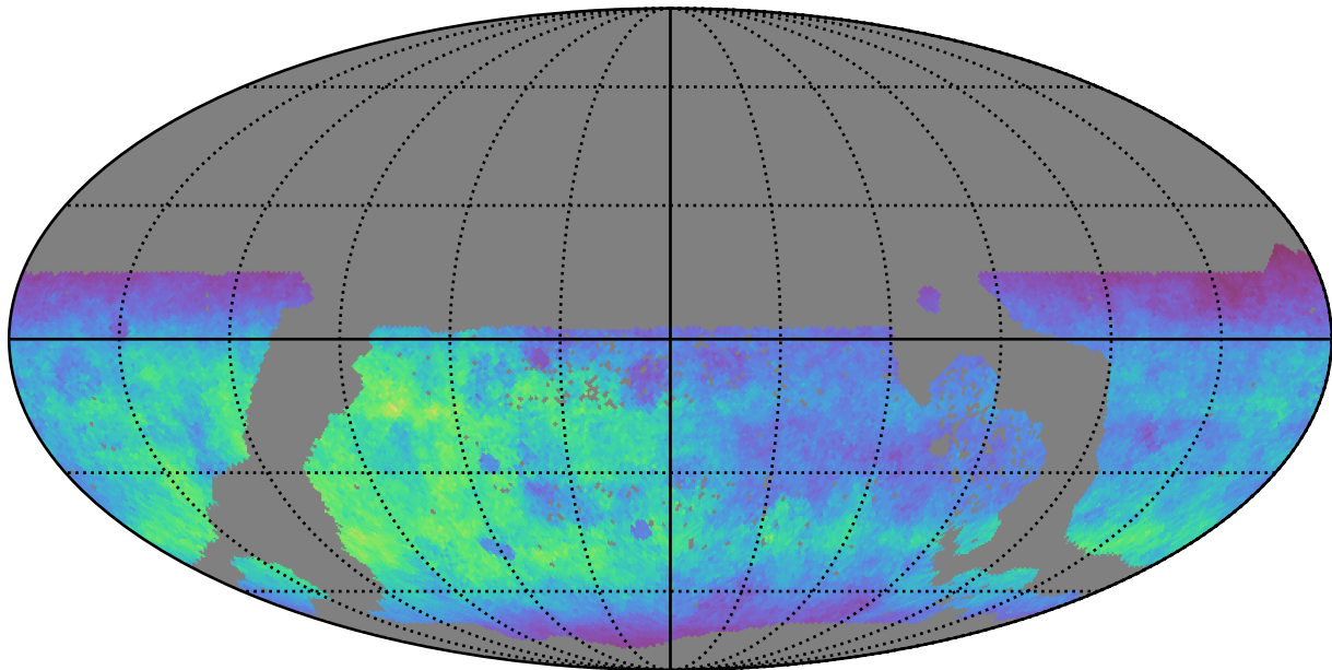
too_elab_r32_d2_gz_v3.4_10yrs WFD g band: Normalized Teff
