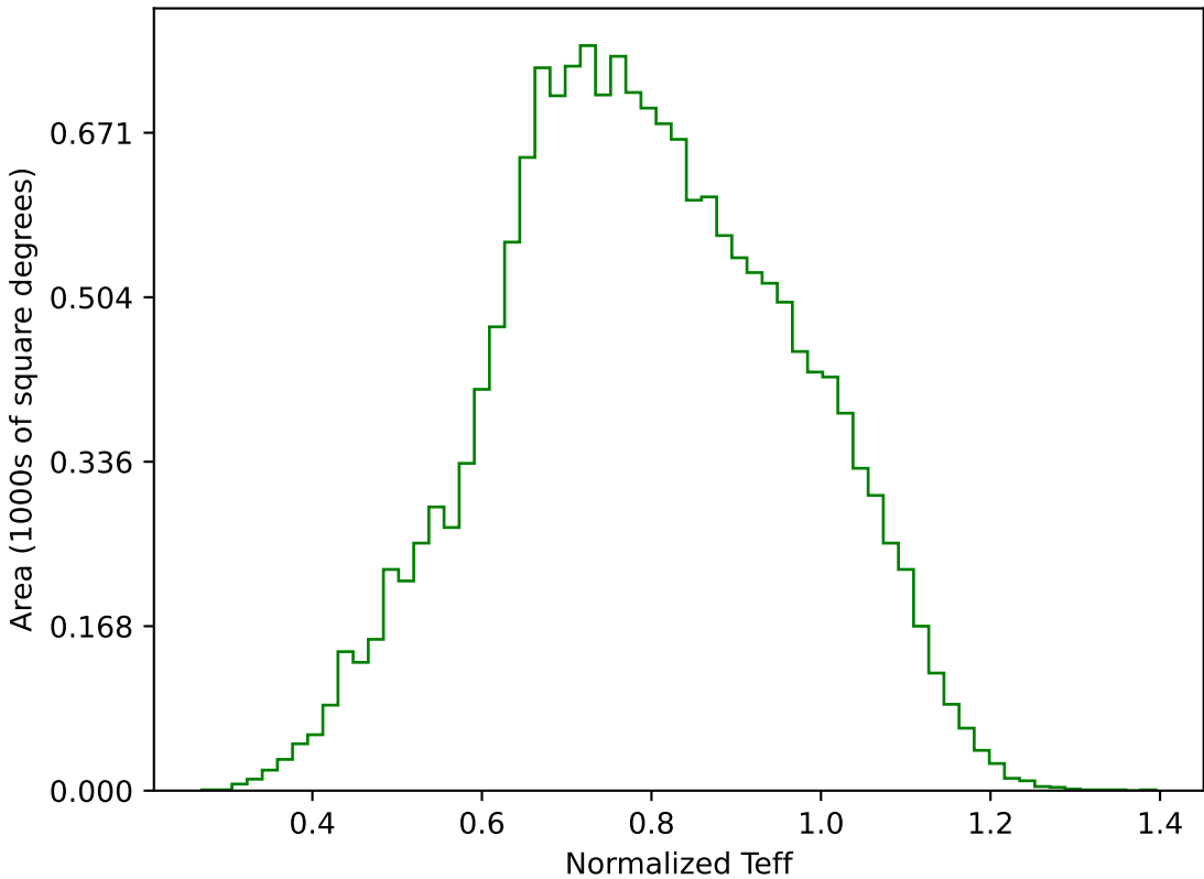
too_elab_r32_d2_gz_v3.4_10yrs WFD g band: Normalized Teff
