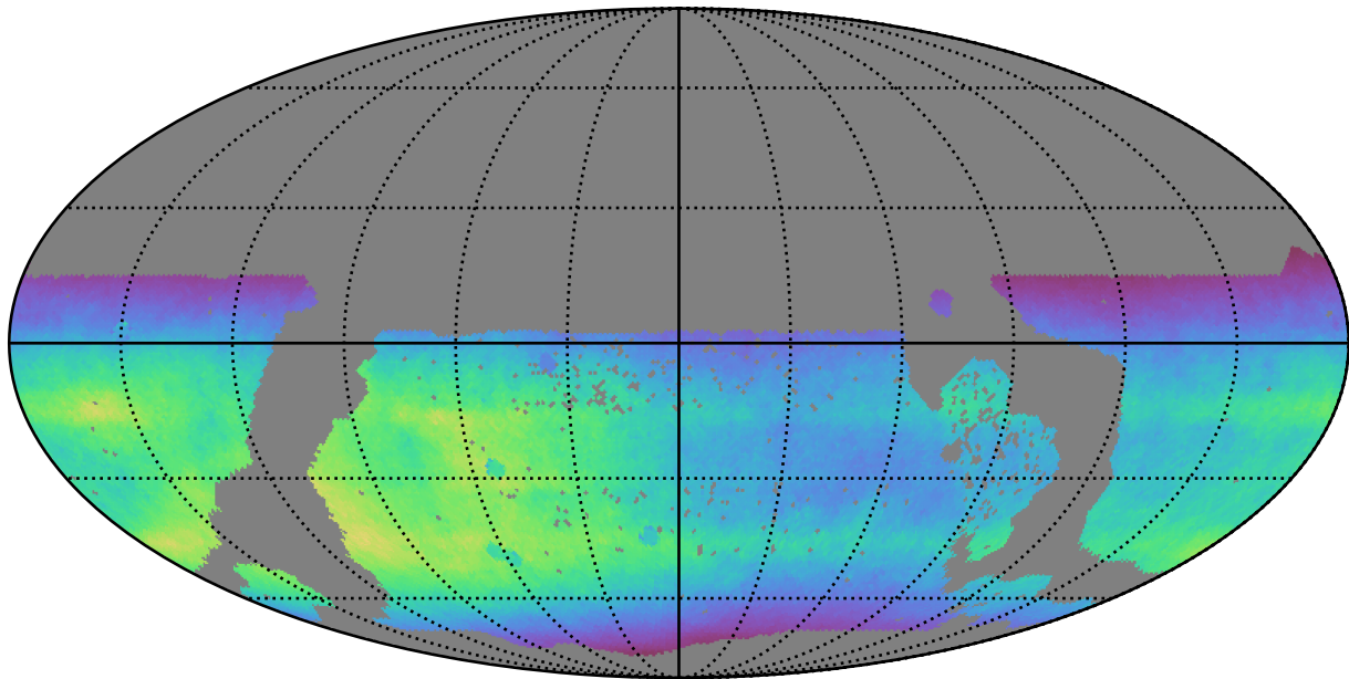
too_elab_r32_d2_gz_v3.4_10yrs WFD all bands: Normalized Teff
