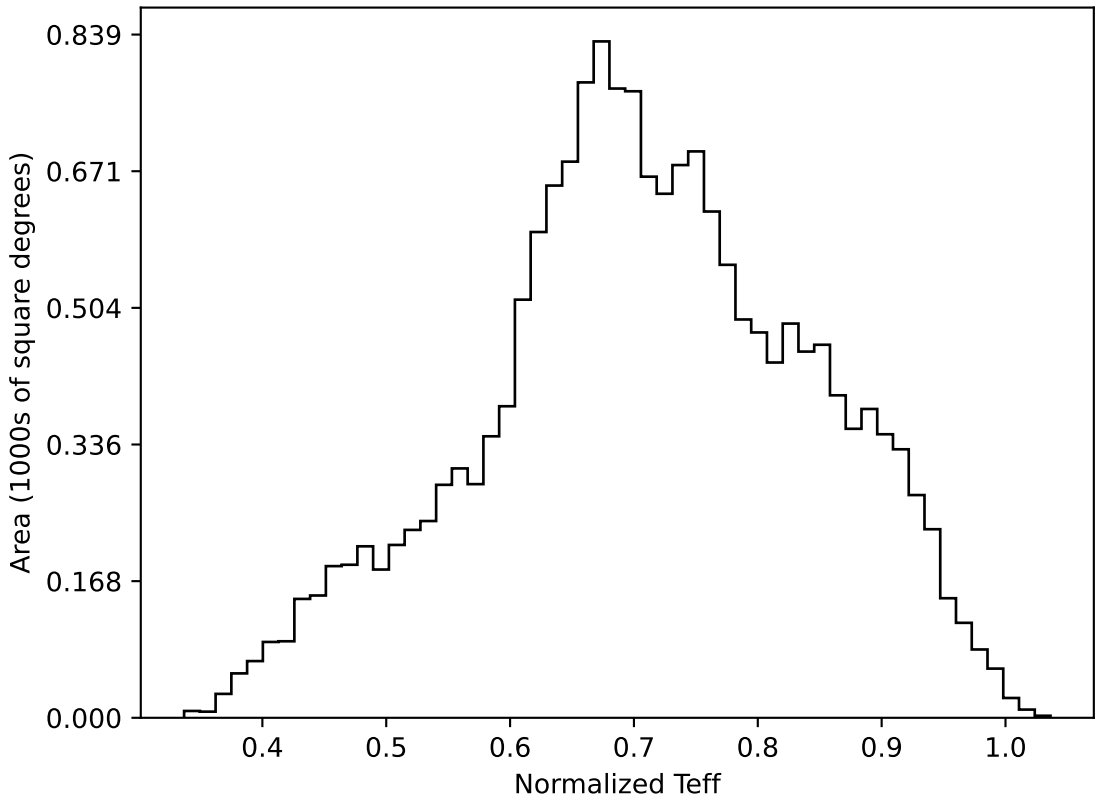
too_elab_r32_d2_gz_v3.4_10yrs WFD all bands: Normalized Teff
