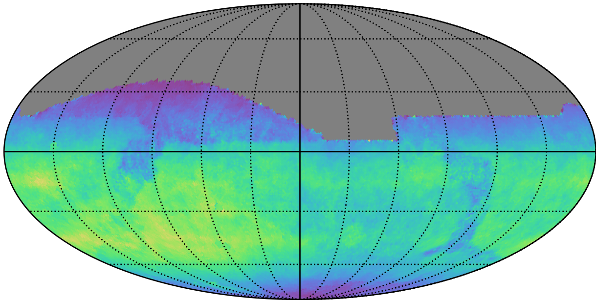
too_elab_r32_d2_gz_v3.4_10yrs All sky z band: Normalized Teff
