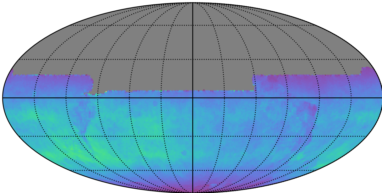
too_elab_r32_d2_gz_v3.4_10yrs All sky y band: Normalized Teff
