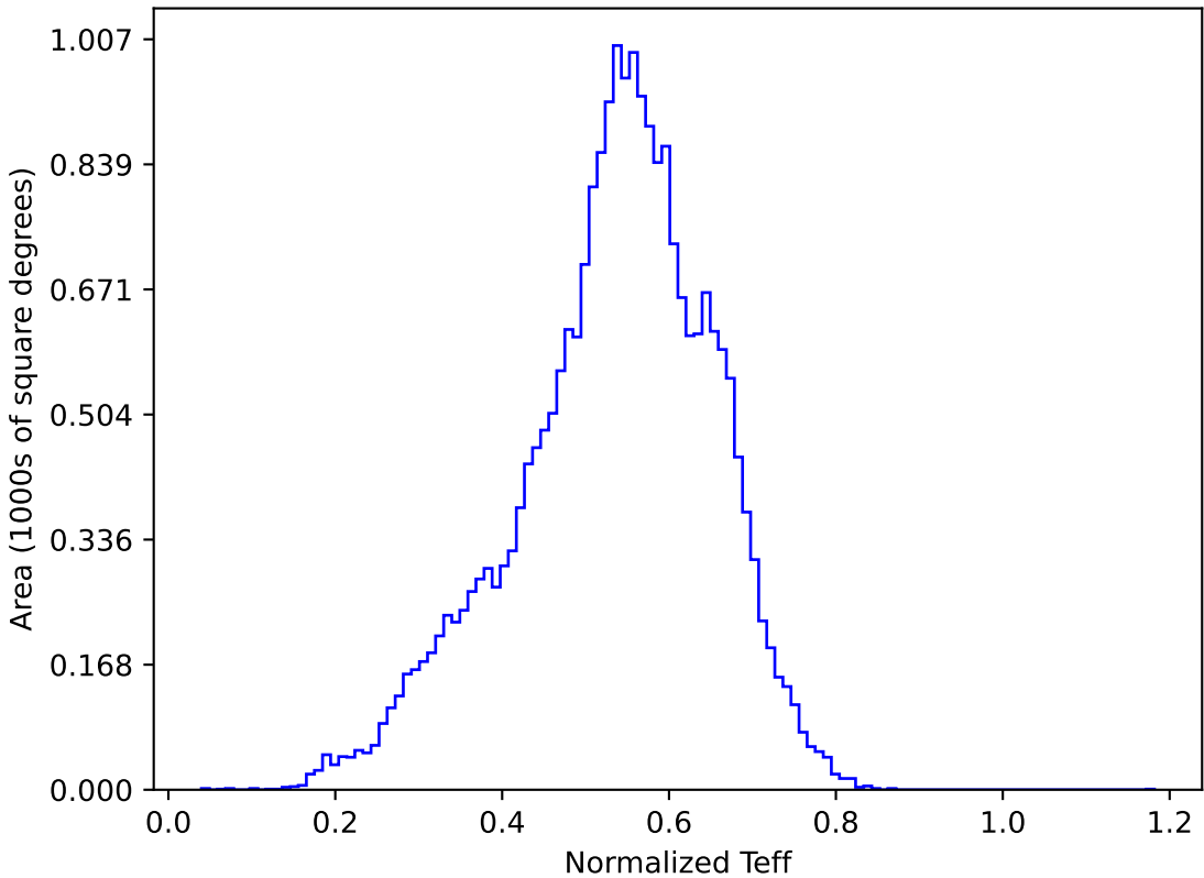
too_elab_r32_d2_gz_v3.4_10yrs All sky y band: Normalized Teff
