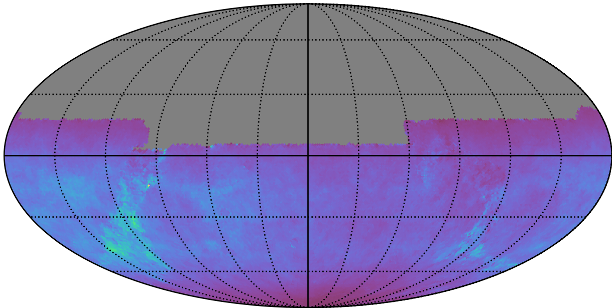
too_elab_r32_d2_gz_v3.4_10yrs All sky u band: Normalized Teff
