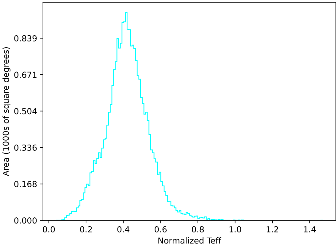
too_elab_r32_d2_gz_v3.4_10yrs All sky u band: Normalized Teff
