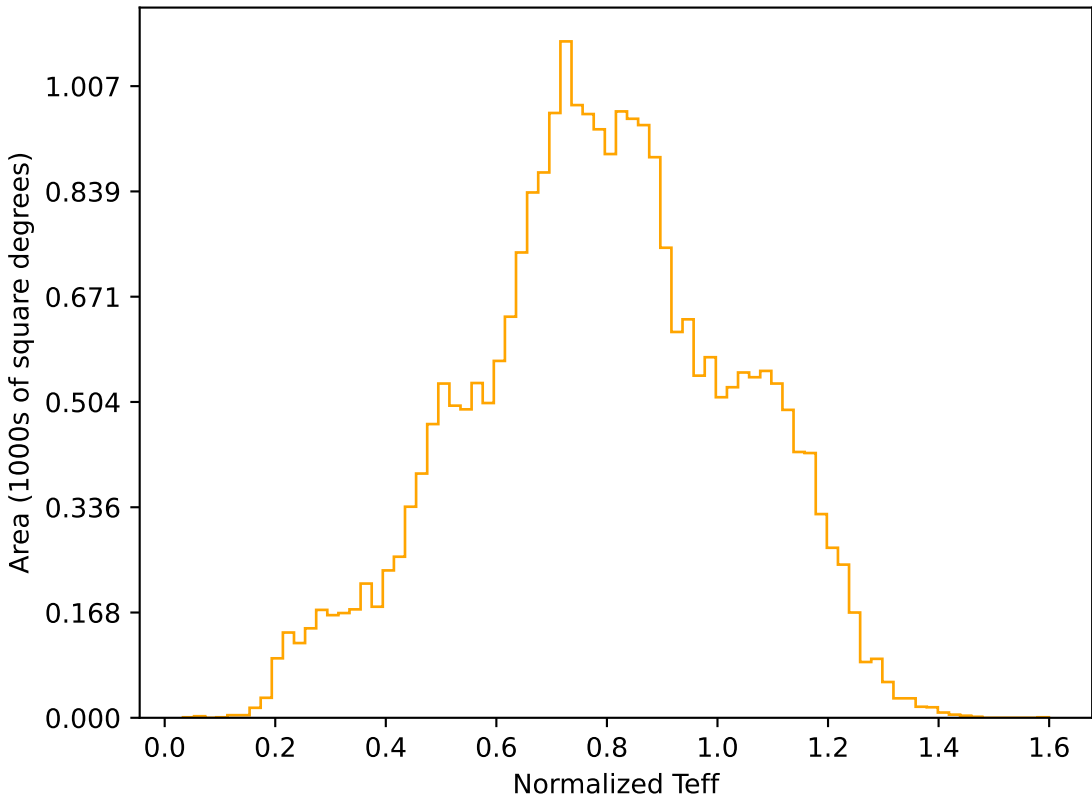
too_elab_r32_d2_gz_v3.4_10yrs All sky r band: Normalized Teff
