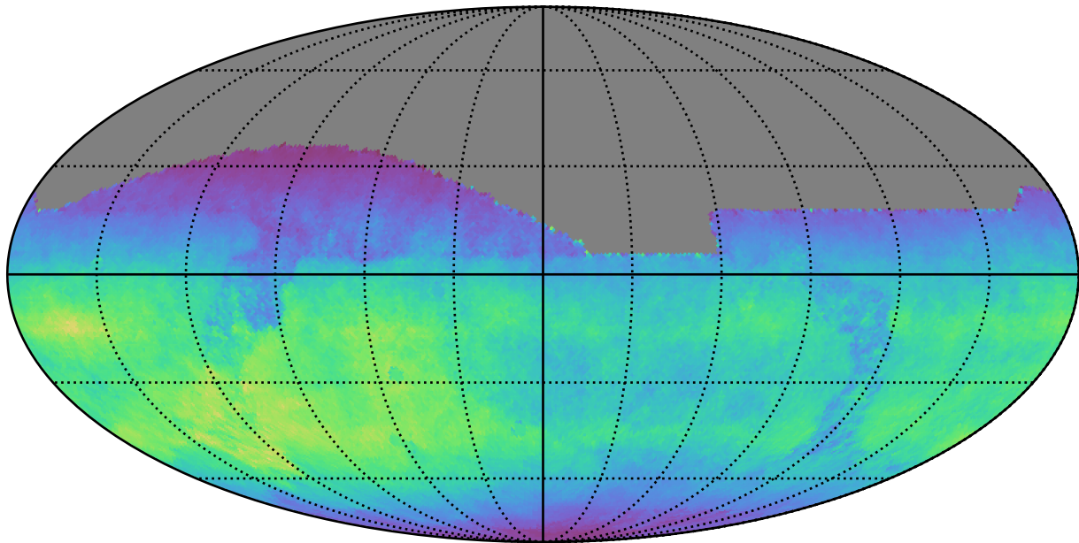
too_elab_r32_d2_gz_v3.4_10yrs All sky i band: Normalized Teff
