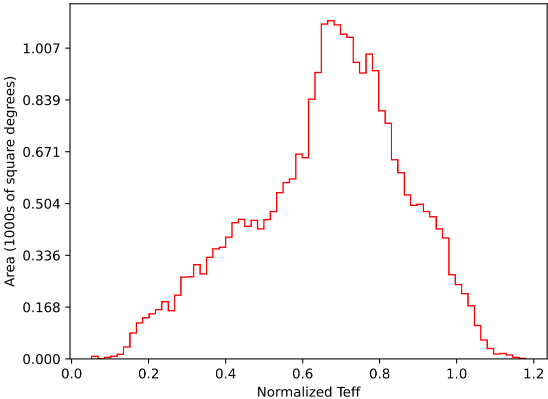
too_elab_r32_d2_gz_v3.4_10yrs All sky i band: Normalized Teff
