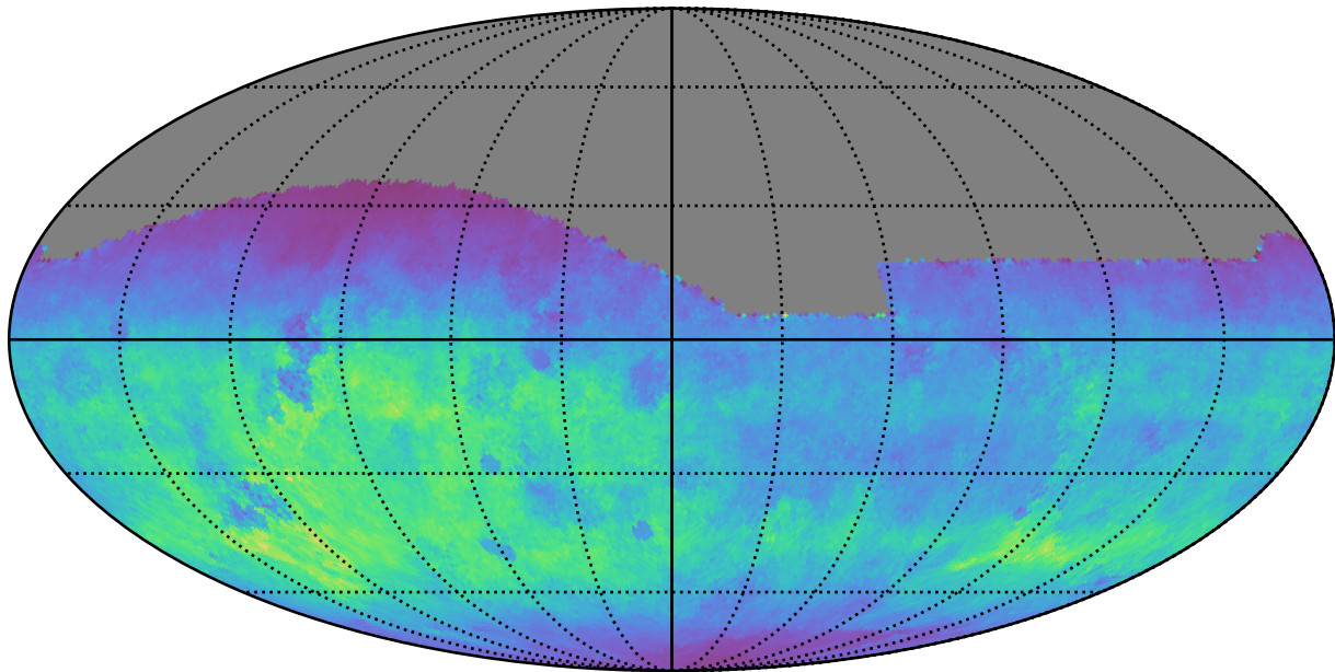
too_elab_r32_d2_gz_v3.4_10yrs All sky g band: Normalized Teff
