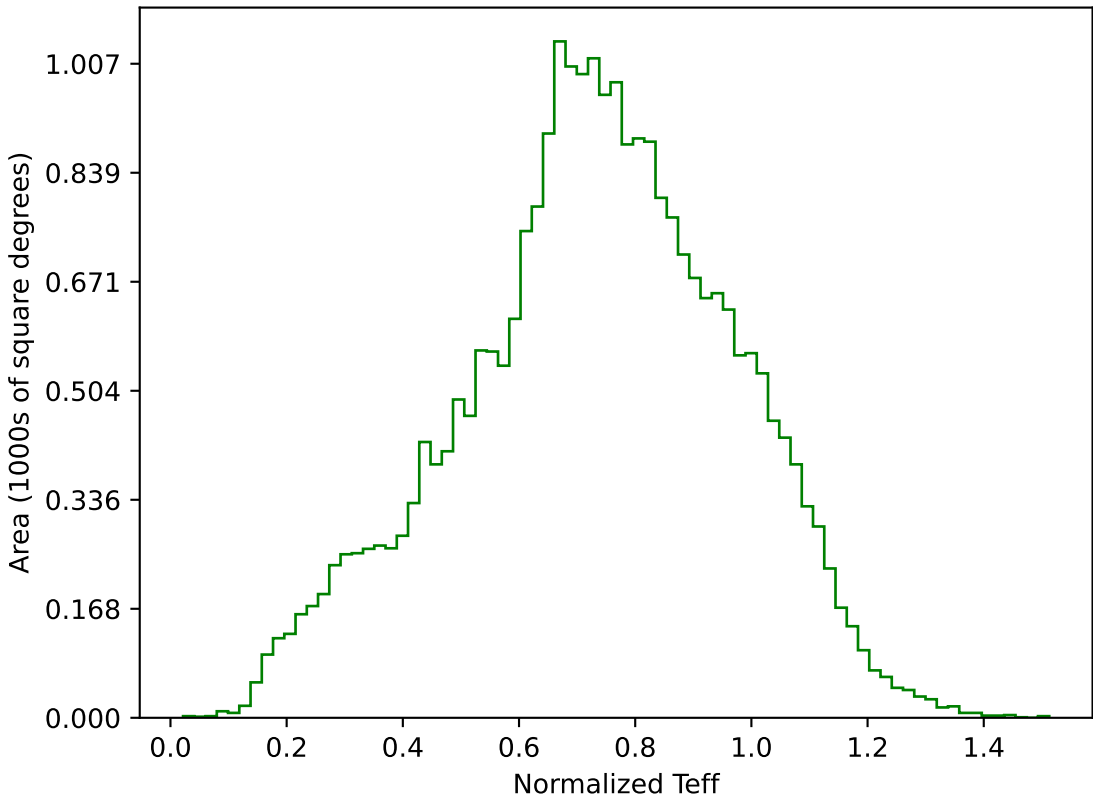
too_elab_r32_d2_gz_v3.4_10yrs All sky g band: Normalized Teff
