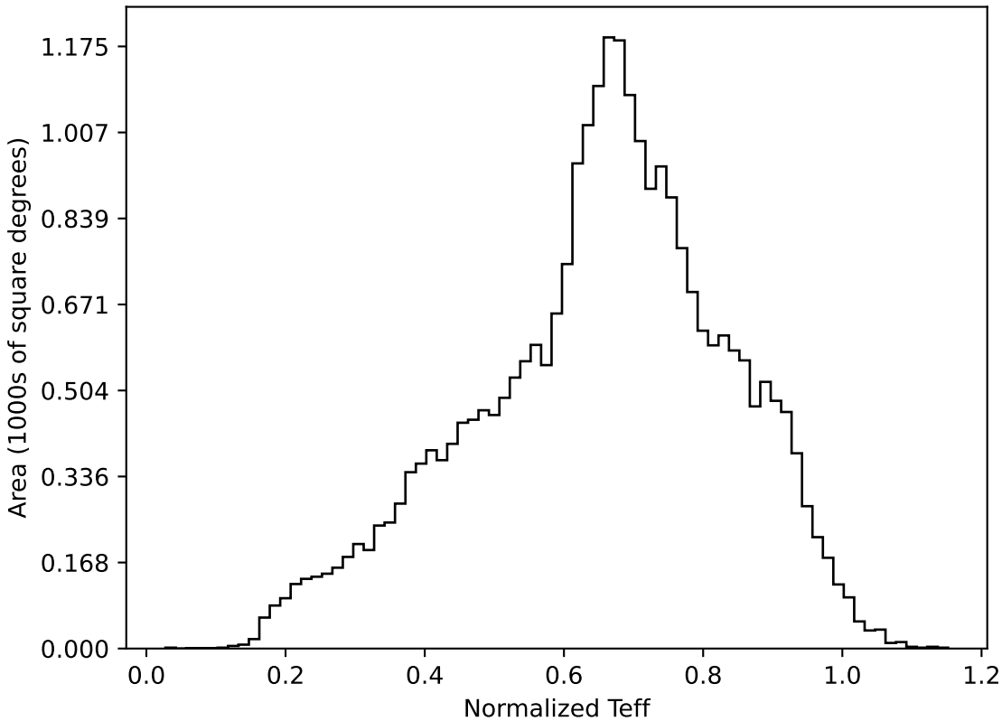
too_elab_r32_d2_gz_v3.4_10yrs All sky all bands: Normalized Teff
