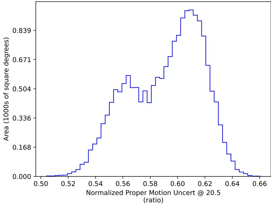
too_elab_r32_d2_gz_v3.4_10yrs WFD: Normalized Proper Motion Uncert @ 20.5
