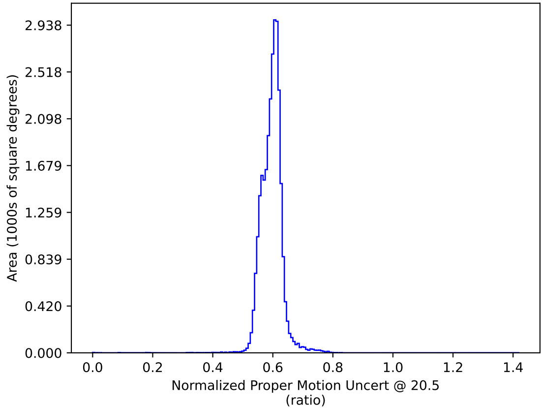
too_elab_r32_d2_gz_v3.4_10yrs All sky: Normalized Proper Motion Uncert @ 20.5
