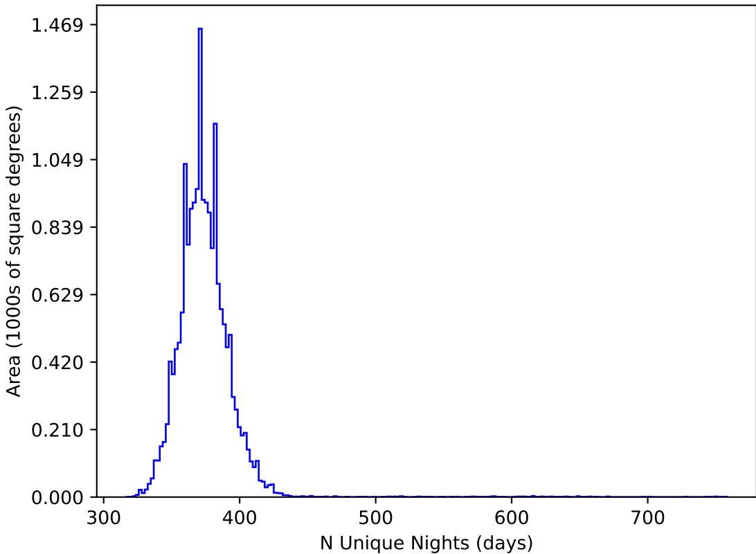
too_elab_r32_d2_gz_v3.4_10yrs WFD all bands: N Unique Nights
