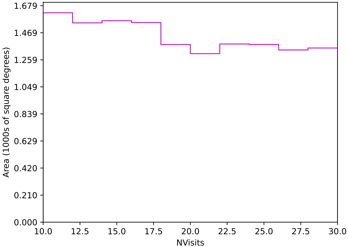
too_elab_r32_d2_gz_v3.4_10yrs Yr 3-4 z band: NVisits
