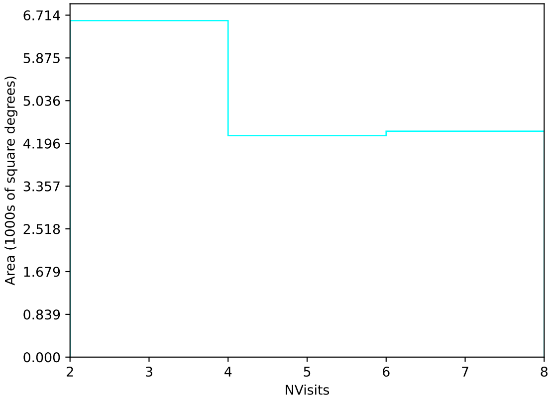
too_elab_r32_d2_gz_v3.4_10yrs Yr 3-4 u band: NVisits
