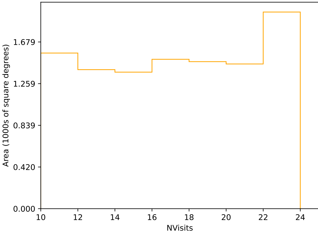
too_elab_r32_d2_gz_v3.4_10yrs Yr 3-4 r band: NVisits
