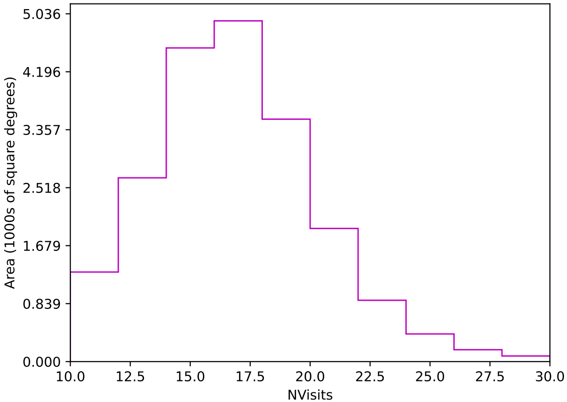
too_elab_r32_d2_gz_v3.4_10yrs Yr 1 z band: NVisits
