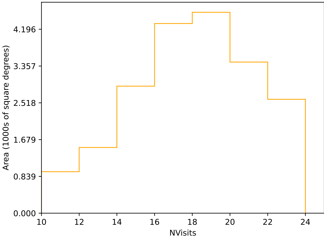
too_elab_r32_d2_gz_v3.4_10yrs Yr 1 r band: NVisits
