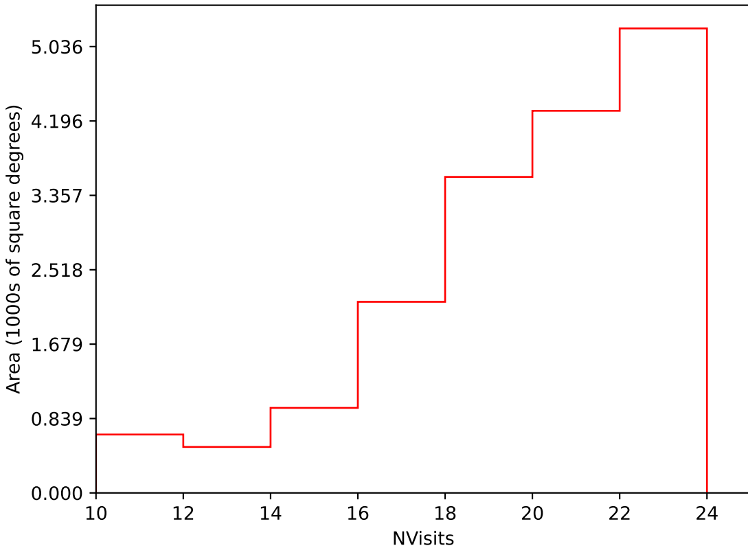
too_elab_r32_d2_gz_v3.4_10yrs Yr 1 i band: NVisits
