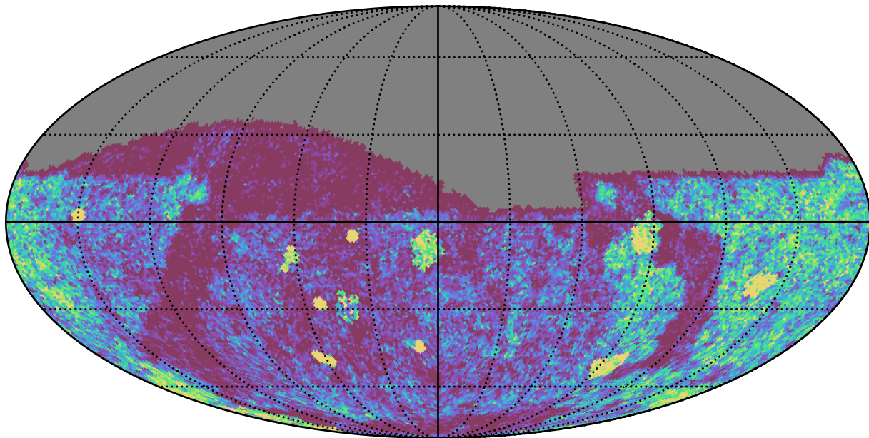
too_elab_r32_d2_gz_v3.4_10yrs Yr 1 g band: NVisits
