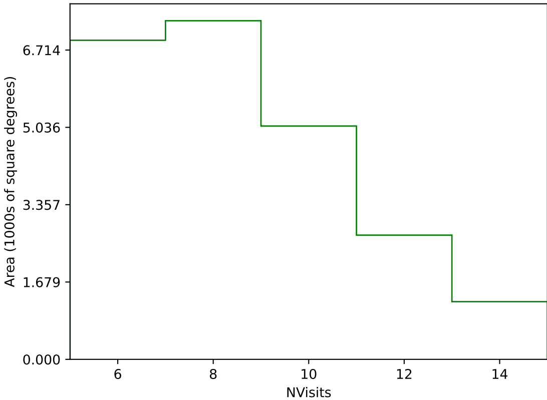
too_elab_r32_d2_gz_v3.4_10yrs Yr 1 g band: NVisits
