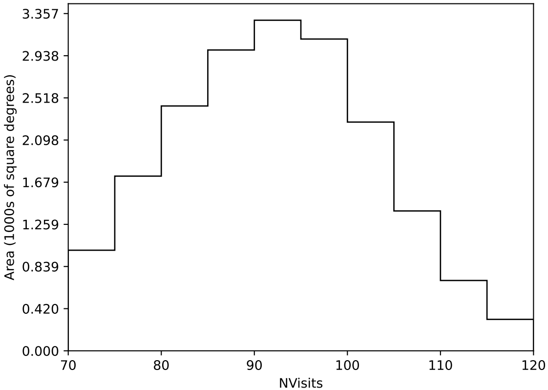
too_elab_r32_d2_gz_v3.4_10yrs Yr 1 all bands: NVisits
