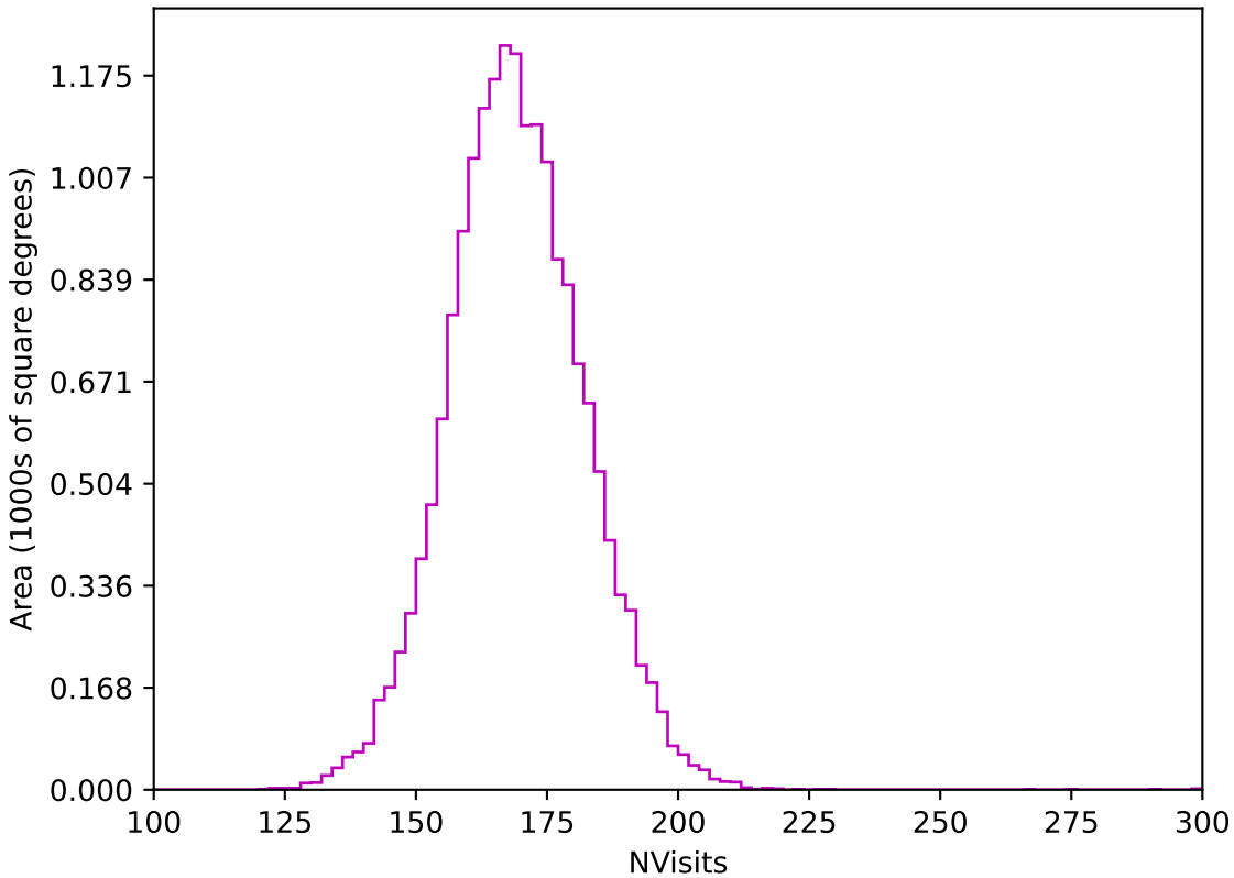
too_elab_r32_d2_gz_v3.4_10yrs WFD z band: NVisits
