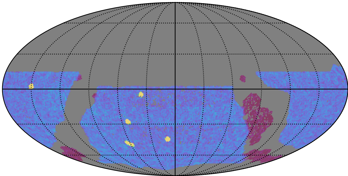
too_elab_r32_d2_gz_v3.4_10yrs WFD y band: NVisits
