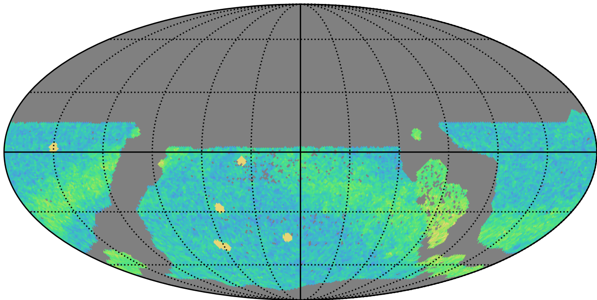
too_elab_r32_d2_gz_v3.4_10yrs WFD r band: NVisits
