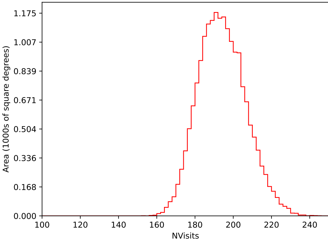
too_elab_r32_d2_gz_v3.4_10yrs WFD i band: NVisits
